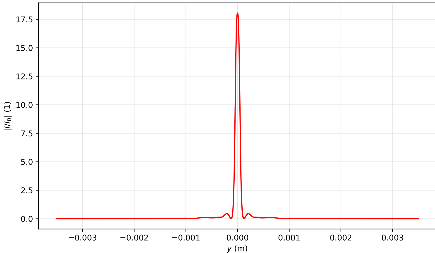
Intensity profile I(x=0, y, z=1.433)/I_0 , P_{in}=6.0P_{cr} , artificial time
